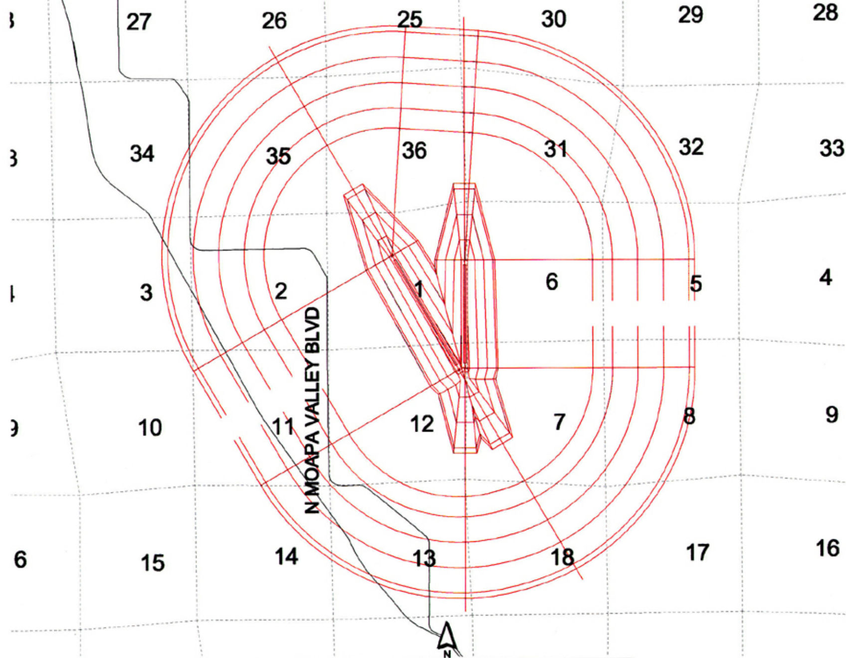
Overton Airport Airspace Map - Appendix G, Map 1F
